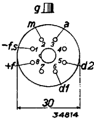
Fig. 2 Arrangement and sequence of contacts.
