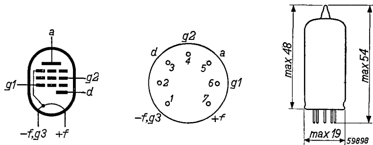
Fig. 2 Electrode arrangement, electrode connections and max. dimensions (in mm) of the DAF 91.
