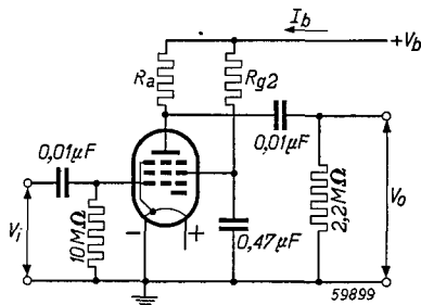
Fig. 3 The DAF 91 used as A.F. amplifier.
