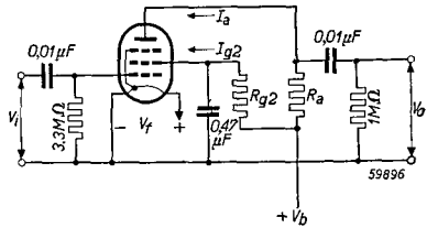
Fig. 3. Circuit diagram showing the DAF 41 used as A.F. amplifier.
