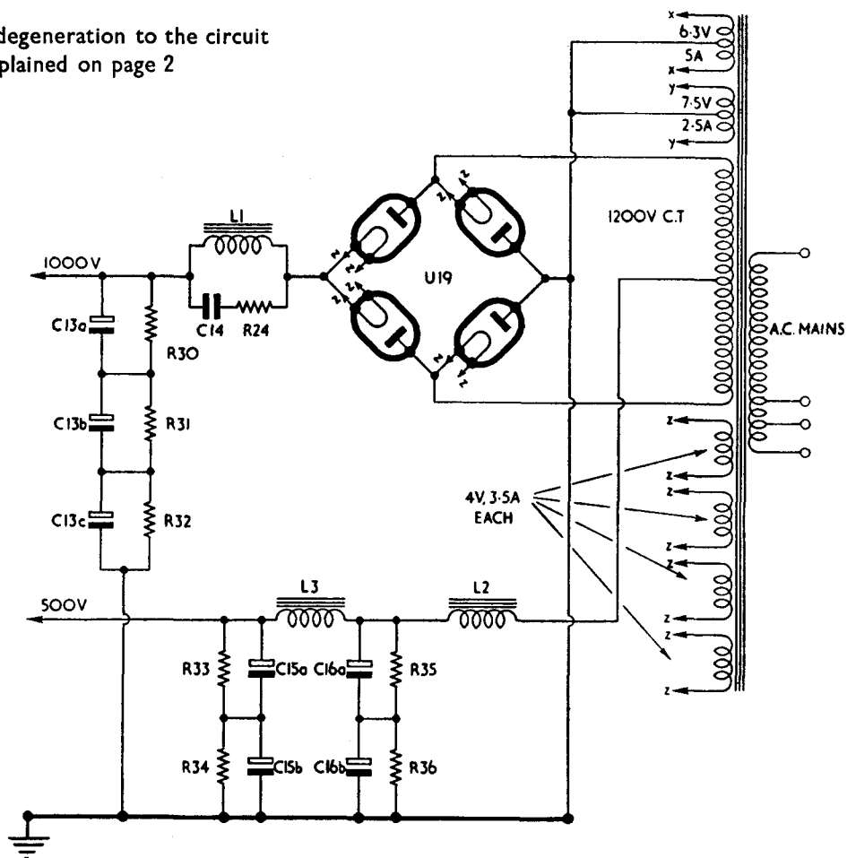
Fig. 6. Power supply unit. Component values are given on page 8
