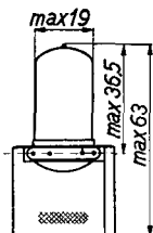
Arrangement of electrodes; connections and maximum dimensions in millimetres.
