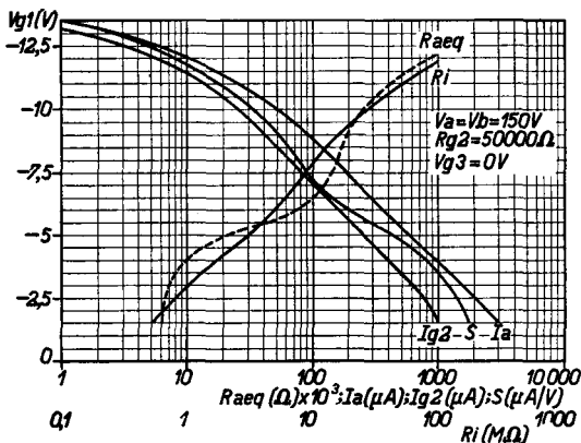
Equivalent noise resistance, anode current, screen-grid current, slope and AC resistance shown against negative grid potential, when the valve is used as RF or IF amplifier with a series-fed screen.
