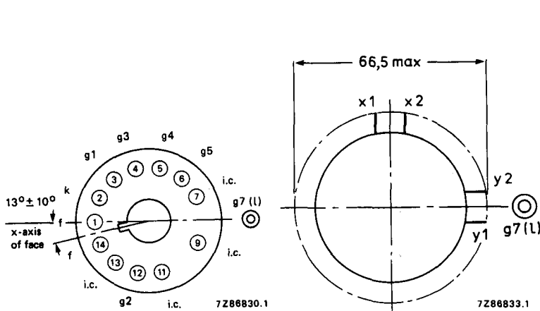
Fig. 2 Pin arrangement; bottom view.
