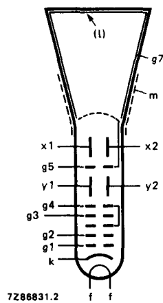
Fig. 4 Electrode configuration.
