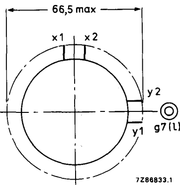
Fig. 3 Side-contact arrangement bottom view.
