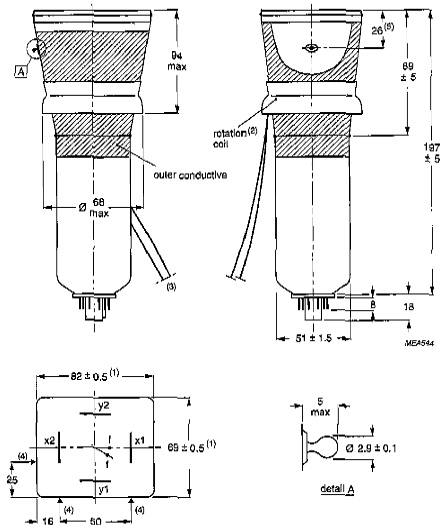
Fig.1 Mechanical outlines.
