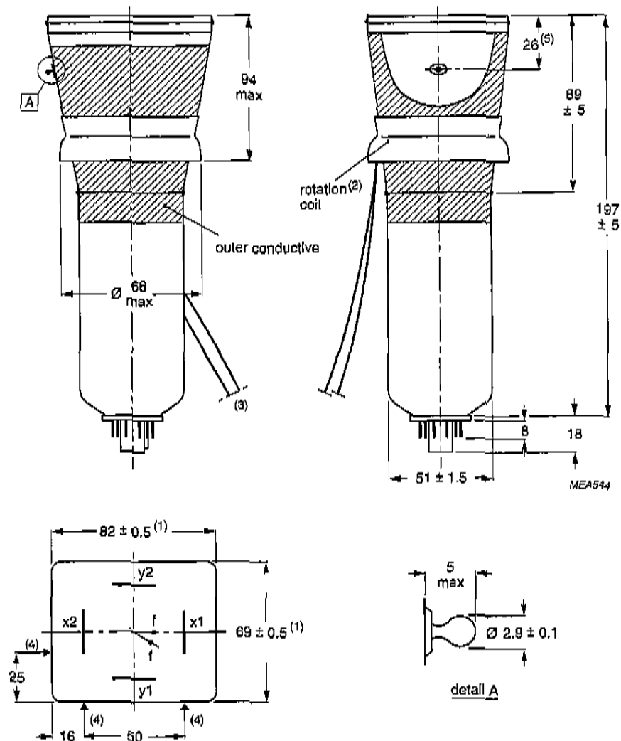
Fig.1 Mechanical outlines.
