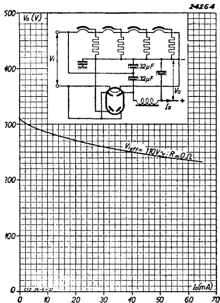
Fig. 4 Loading characteristic of the CY 2 used as a voltage doubler. This curve also applies to both voltage-doubling circuits
