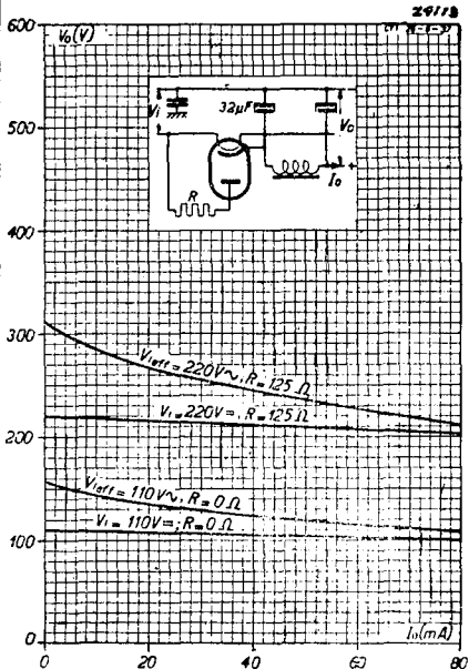
Fig. 3 Loading characteristics of the CY 1.
