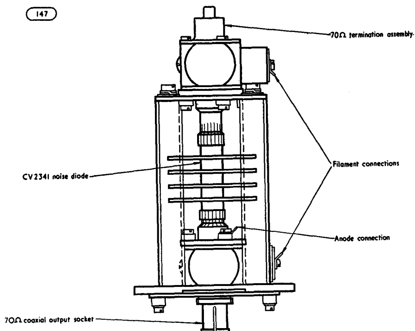
Fig. 3. External view of a typical circuit.
