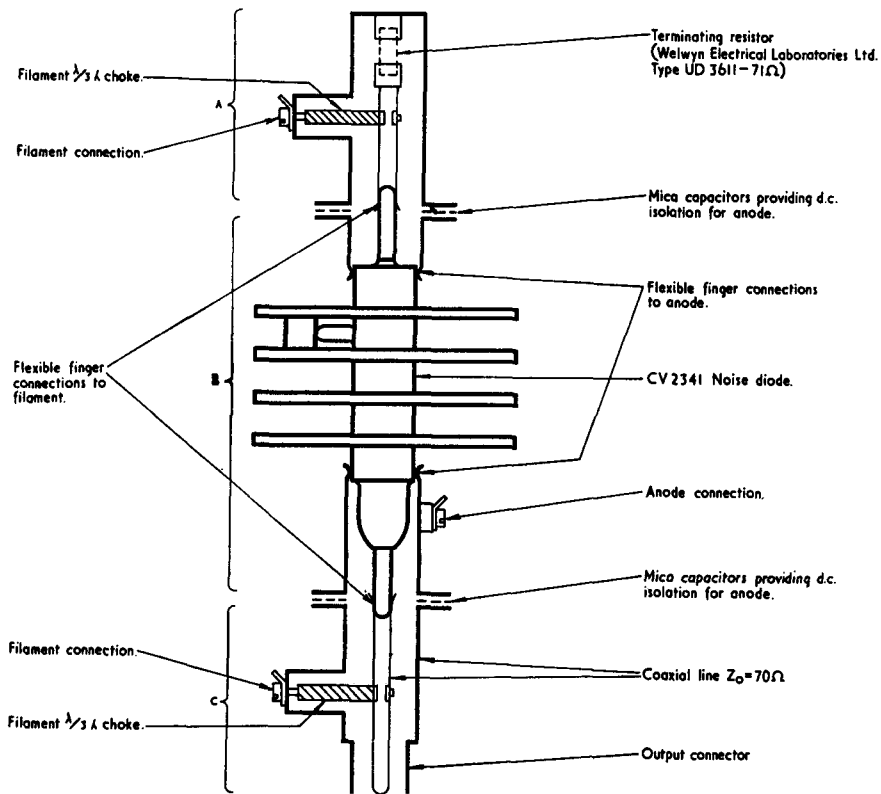
Fig. 2. Diagrammatic section through coaxial noise diode circuit.
