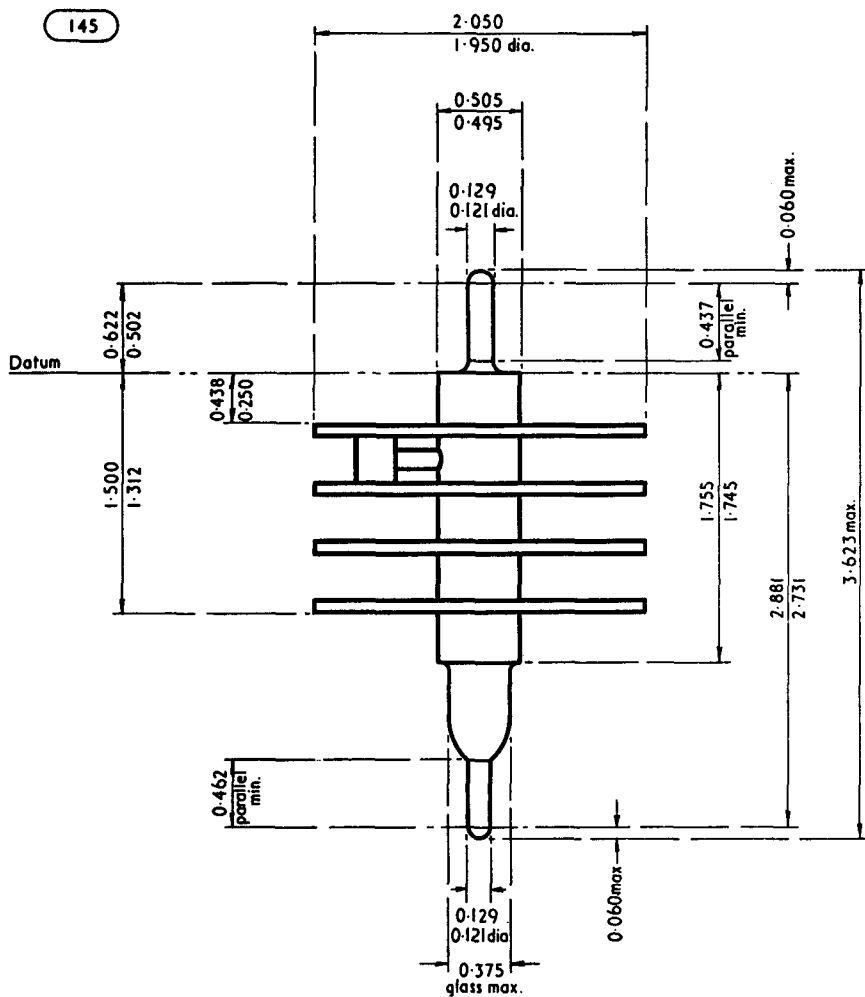
Fig. 1. Dimensions in inches.
