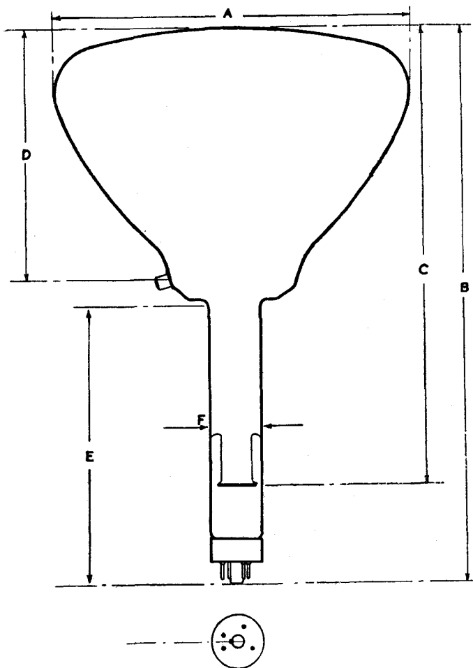
OUTLINE DRAWING OF CRM 91
