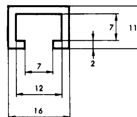
Positioning rail
