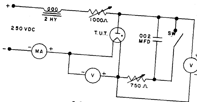
D.C. TEST CIRCUIT
