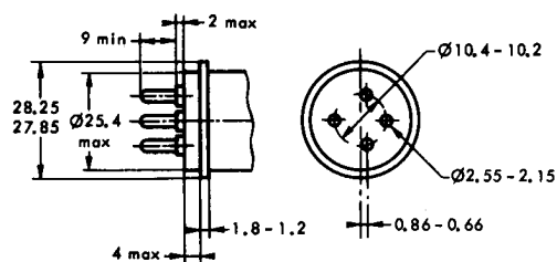
Pin arrangement
