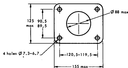
Water connection
