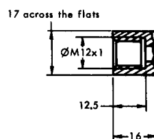
Water connection
