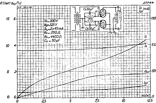
Fig. 12 Anode current I_a , screen-grid current I_{g2} , total distortion d_{tot} and alternating grid voltage V_i as functions of the output power W_0 for two CL 6 valves in a balanced circuit with V_a = 200 V, and V_{g2} = 125 V.
