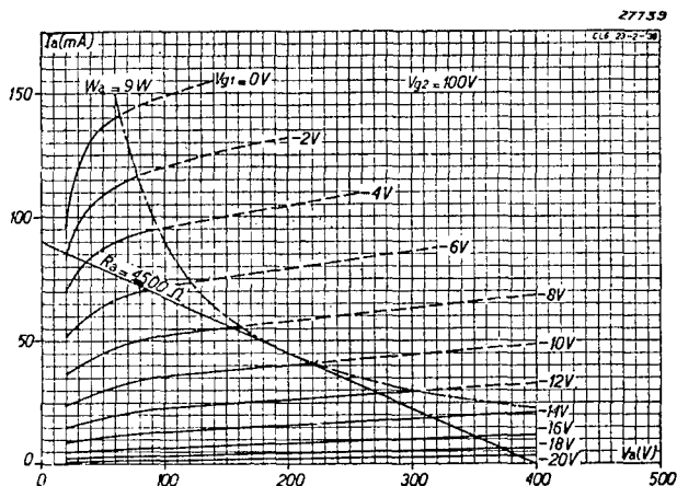
Fig. 4 Anode current as a function of the anode voltage at V_{g2} = 100 V, with grid bias as parameter.
