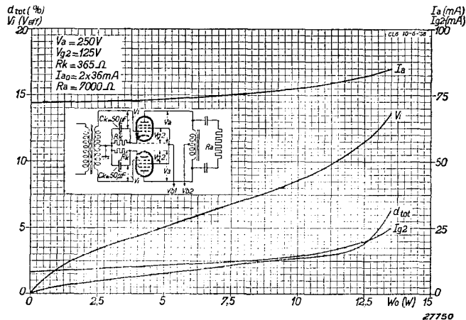
Fig. 13 Anode current I_a , screen current I_{g2} , total distortion d_{tot} and alternating grid voltage V_i as functions of the output power for two type CL 6 valves in a balanced circuit with V_a = 250 V, and V_{g2} = 125 V.
