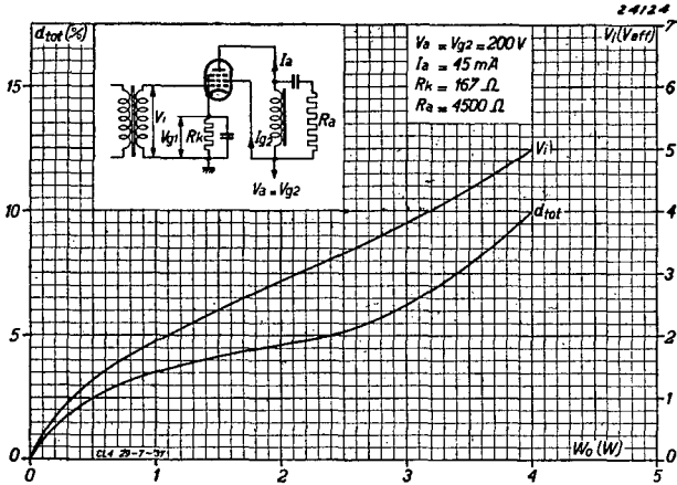
Fig. 5 Alternating grid voltage and total distortion as functions of the output power of the CL 4 when used as a single output valve.
