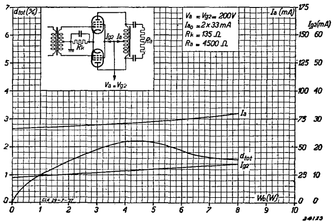
Fig. 6 Anode current, screen current and total distortion as functions of the output power for two CL 4 valves in a balanced output stage.
