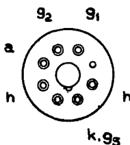
OCTAL BASE
