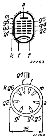
Fig. 2 Arrangement of electrodes and base connections.
