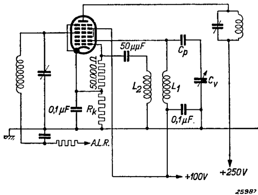
Fig. 8 Oscillator anode fed through the tuning coil. This arrangement is suitable for 100 V supply but has the disadvantage that the padding capacitors for the different wave ranges have to be switched.
