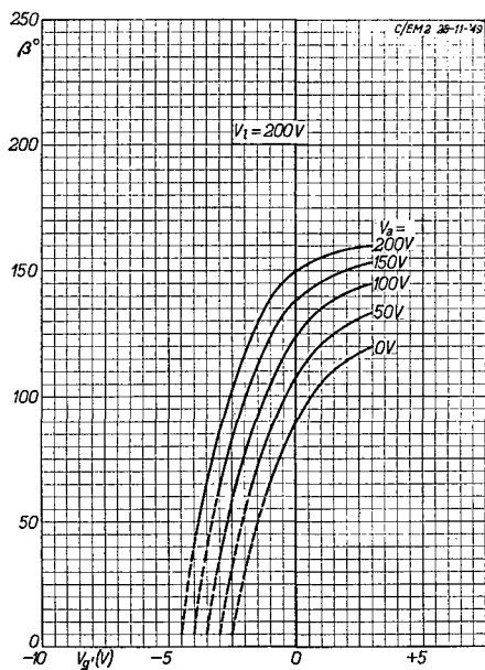
Fig. 9 Light angle \beta of the fluorescent screen as a function of the voltage V_{g'} on the grid of the indicator section, with the voltage V_a on the anode of the triode as parameter. Voltage V_l on the fluorescent screen constant at 200 V.
