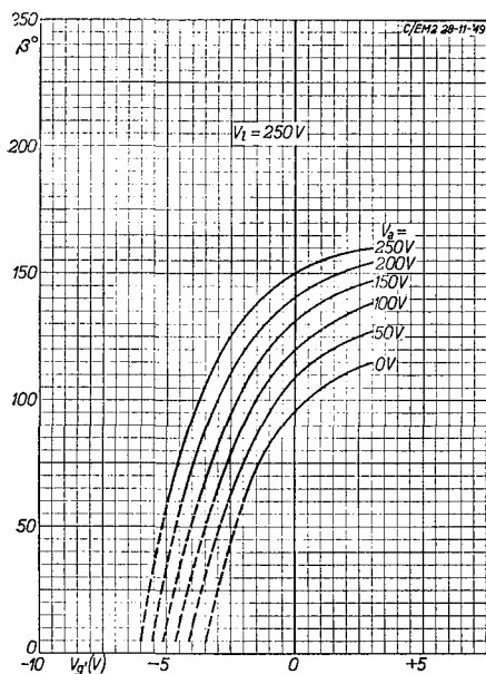
Fig. 8 Light angle \beta of the fluorescent screen as a function of the voltage V_{g'} on the grid of the indicator section, with the voltage V_a on the anode of the triode as parameter. Voltage V_l on the fluorescent screen constant at 250 V.
