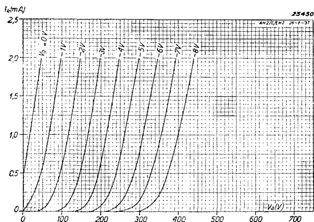
Fig. 5 Triode section of the C/EM 2. Anode current as a function of the anode voltage for various values of grid bias, reproduced on a small anode-current scale.
