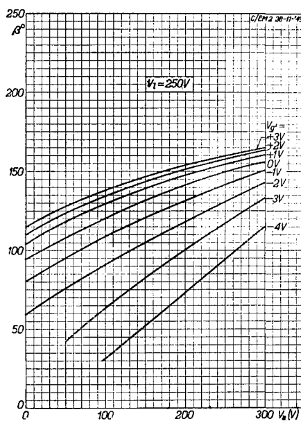
Fig. 6 Light sector angle \beta of the fluorescent screen as a function of the anode voltage V_a of the triode section, with the grid bias V_g of the indicator section as parameter. The broken lines on the curve indicate the range in which the light sectors decrease in size. Voltage V_1 on the screen constant at 250 V.
