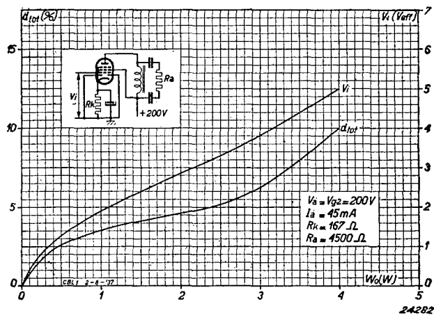
Fig. 5 Alternating grid voltage and total distortion as functions of the output power.
