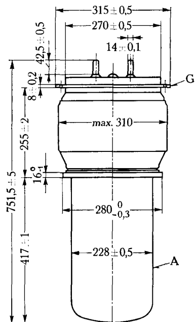
BTW 150-2
