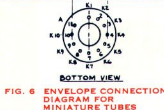
FIG. 6 ENVELOPE CONNECTION DIAGRAM FOR MINIATURE TUBES
