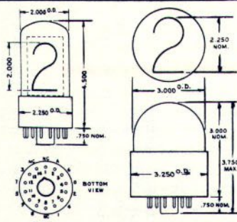
FIG. 4 OUTLINE DRAWING FOR JUMBO TUBES
