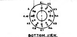
FIG. 6 ENVELOPE CONNECTION DIAGRAM FOR MINIATURE TUBES
