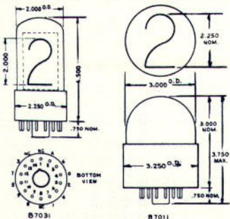
FIG. 4 OUTLINE DRAWING FOR JUMBO TUBES
