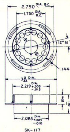
FIG. 10 CONTACT SOCKET ASSEMBLY SK 117 FOR JUMBO TUBES
