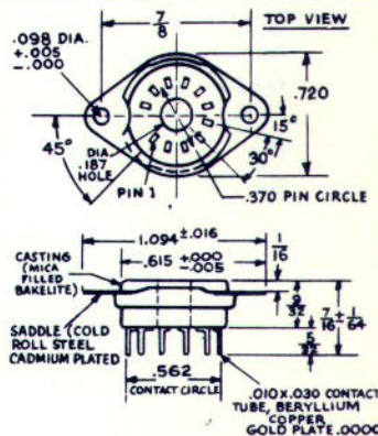
FIG. 9 CONTACT SOCKET ASSEMBLY SK 116 FOR MINIATURE TUBES
