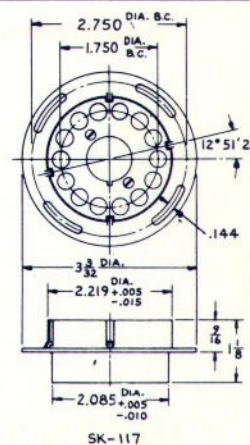
FIG. 10 CONTACT SOCKET ASSEMBLY SK 117 FOR JUMBO TUBES
