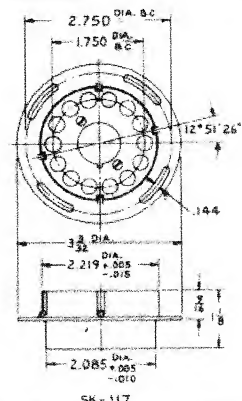
FIG. 10 CONTACT SOCKET ASSEMBLY SK 117 FOR JUMBO TUBES
