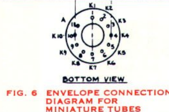
FIG. 6 ENVELOPE CONNECTION DIAGRAM FOR MINIATURE TUBES
