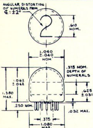
FIG. 1 OUTLINE DRAWING FOR STANDARD TUBES
