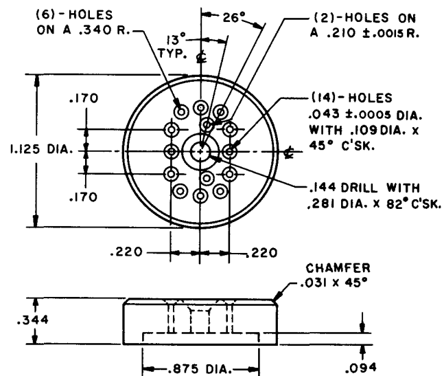
PIN STRAIGHTENER
