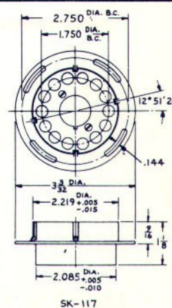
FIG. 10 CONTACT SOCKET ASSEMBLY SK 117 FOR JUMBO TUBES
