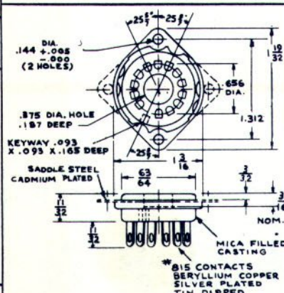
FIG. 8 CONTACT SOCKET ASSEMBLY HSK 106 AND HSK 112 FOR STANDARD AND SUPER TUBES
