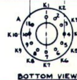
FIG. 6 ENVELOPE CONNECTION DIAGRAM FOR MINIATURE TUBES
