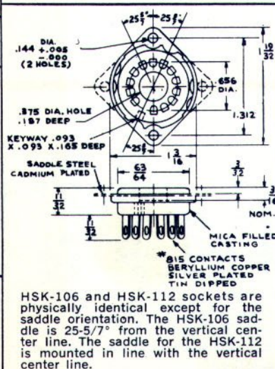
FIG. 8 CONTACT SOCKET ASSEMBLY HSK 106 AND HSK 112 FOR STANDARD AND SUPER TUBES
