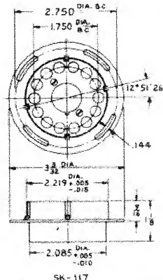
FIG. 10 CONTACT SOCKET ASSEMBLY SK 117 FOR JUMBO TUBES
