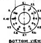
FIG. 6 ENVELOPE CONNECTION DIAGRAM FOR MINIATURE TUBES
