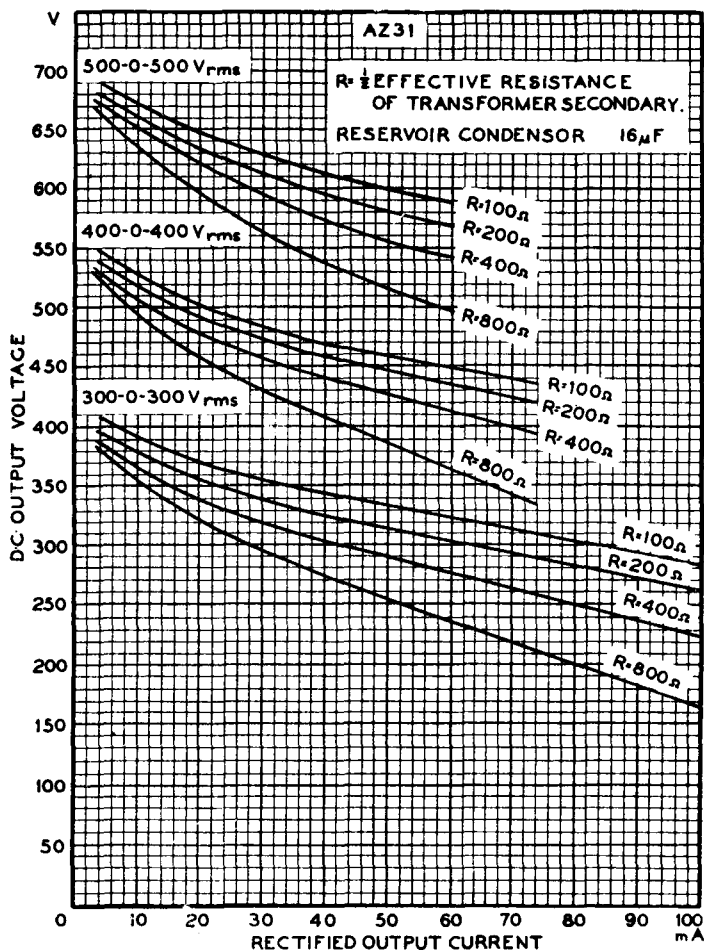
RECTIFIER CHARACTERISTICS
