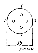
Fig. 2 Arrangement of electrodes and base connections
