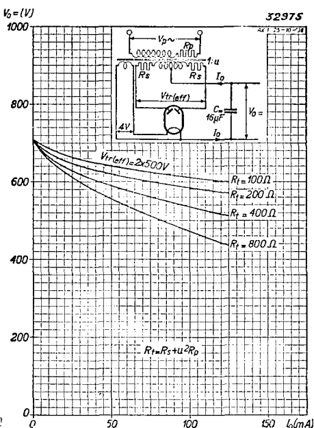
Fig. 4 Loading curves (D.C. voltage as a function of the delivered current) for various values of the total resistance R_t = (R_s + n^2 R_p) , in a smoothing circuit commencing with a capacitor.
