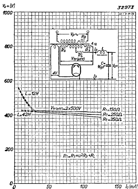
Fig. 3 Loading curves (D.C. voltage as a function of the current delivered) for various values of the resistance R_t = (R_L + R_s + n^2 R_p) , in a smoothing circuit commencing with a choke. The voltages at lower current values with a choke of 12 or 42 henries are shown by broken lines.
