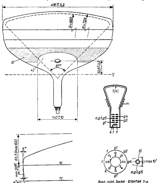
Base, culot, Socket: EIGHTAR 7-p
