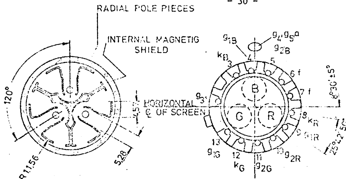
LOCATION OF RADIAL- CONVERGING POLE PIECES
