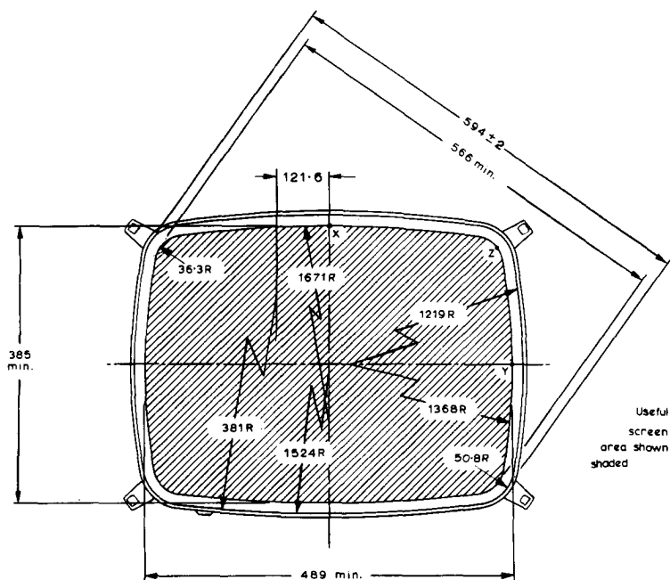
Bulb dimensions
