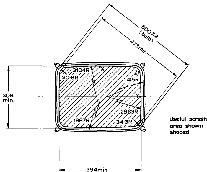
Bulb dimensions
