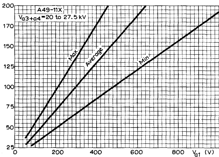
CUT-OFF DESIGN CHART
