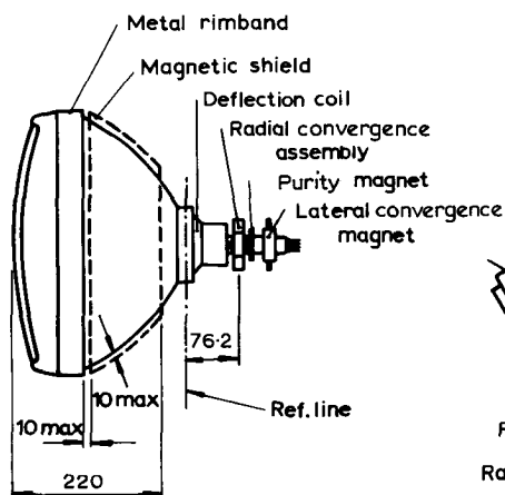
Outline of tube with components
