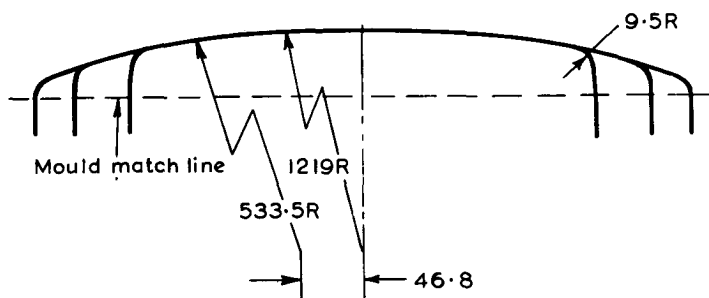
External screen radii
