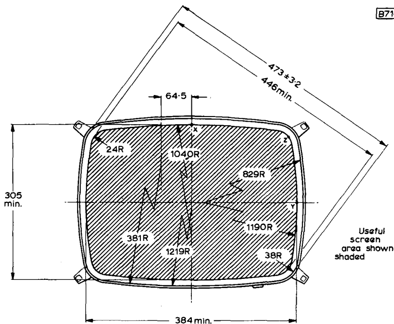
Bulb dimensions
