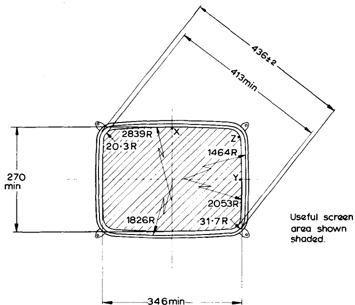
Bulb dimensions
