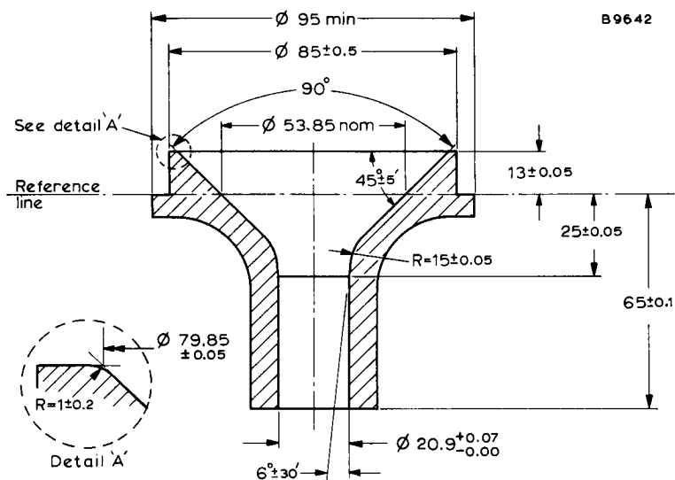
REFERENCE LINE GAUGE All dimensions in mm
