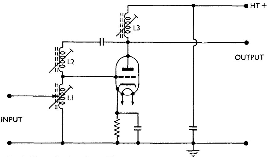
Fig. 1. Neutralised R.F. amplifier.
