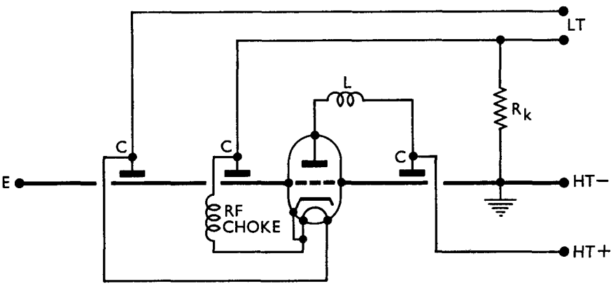
Fig. 2. R.F. oscillator using lumped circuit.
