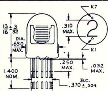
FIG. 3 OUTLINE DRAWING FOR MINIATURE TUBES
