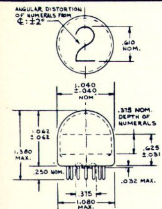
FIG. 1 OUTLINE DRAWING FOR STANDARD TUBES
