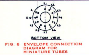
FIG. 6 ENVELOPE CONNECTION DIAGRAM FOR MINIATURE TUBES
