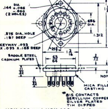
FIG. 8 CONTACT SOCKET ASSEMBLY HSK 106 AND HSK 112 FOR STANDARD AND SUPER TUBES
