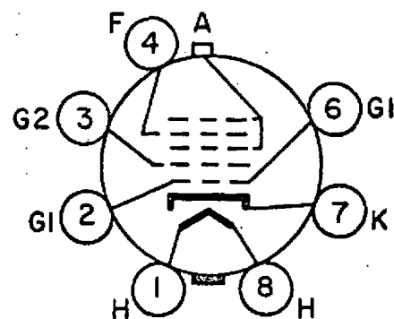
BASING DIAGRAM 8MC
