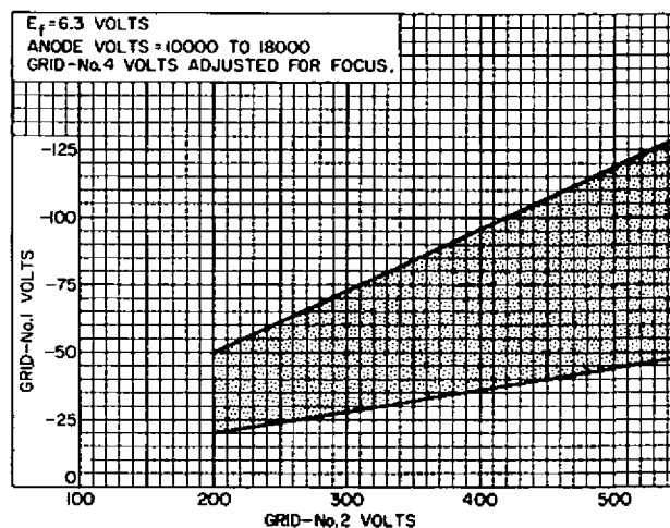
Fig. 2 - Raster-Cutoff Range Chart for Type 8NP4.
